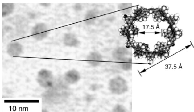
Figure 2. Transmission electron micrograph of \mathbf{18}^{+12} \cdot 12\text{PF}_6^- (magnification of 200 000 \times ) showing an individual, regular hexagon along with its computer generated CPK model for comparison. Darkened metal centers in hexameric arrangement can be observed.
