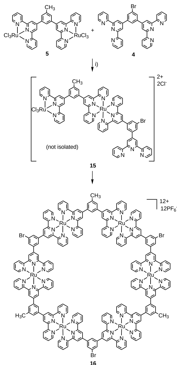
Scheme 6. Synthesis of heteroleptic metallomacrocycle 16 by self-assembly: i) a) N -ethylmorpholine, MeOH, 12 h, reflux, b) methanolic \text{NH}_4^+\text{PF}_6^- .
