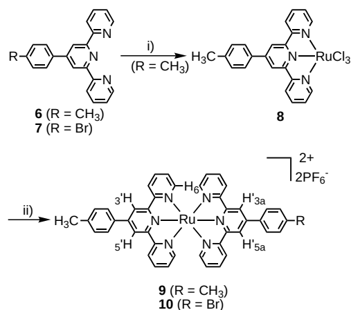
Scheme 2. Synthesis of mono( \text{Ru}^{\text{II}} ) complexes 9 and 10 : i) \text{RuCl}_3 \cdot 3\text{H}_2\text{O} , EtOH, 12 h, reflux; ii) a) N -ethylmorpholine, MeOH, 12 h, reflux, b) methanolic \text{NH}_4^+\text{PF}_6^- .
