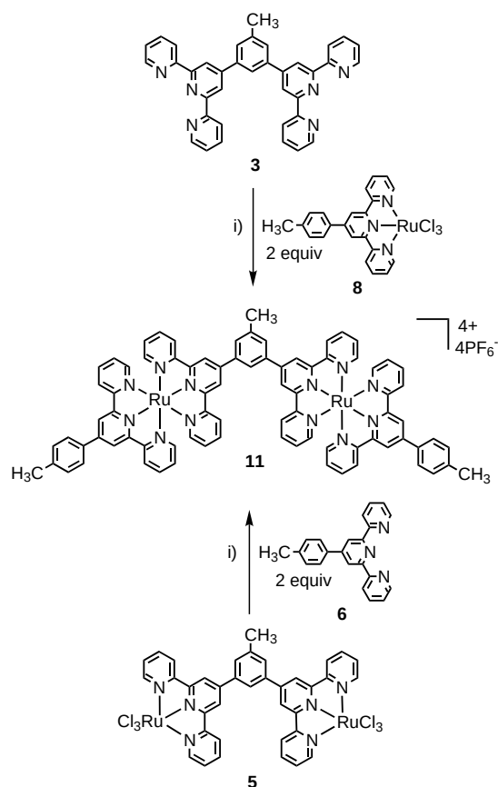
Scheme 3. Synthesis of complex 11 by different routes to verify the structure of bis(Ru III ) adduct 5 ; i) a) N -ethylmorpholine, MeOH, 12 h, reflux, b) methanolic NH 4 + PF 6 − .
