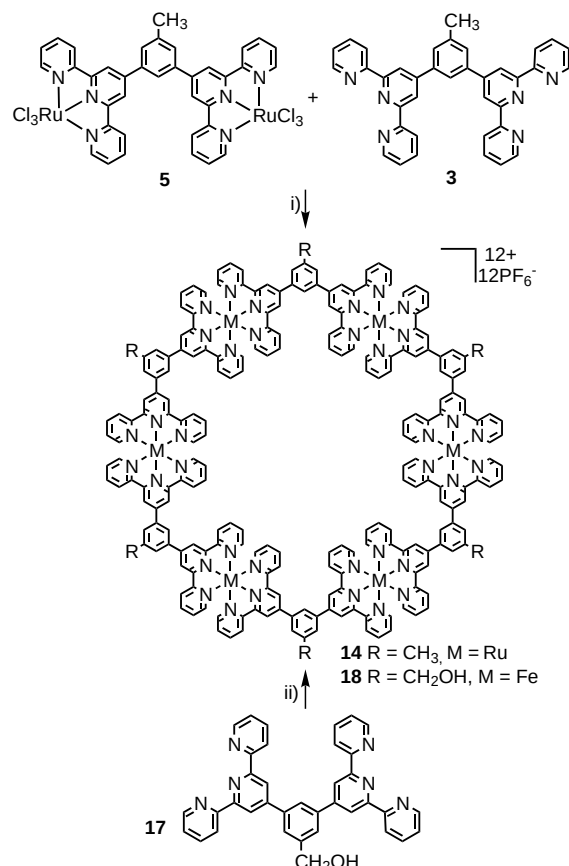
Scheme 4. Synthesis of metallomacrocycles 14 by self- and directed-assembly; i) a) N -ethylmorpholine, MeOH, 12 h, reflux, b) methanolic NH 4 + PF 6 − .
