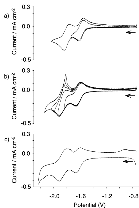
Figure 1. Cyclic voltammograms of 1 mM solutions of a) mono( \text{Ru}^{\text{II}} ) complex 9 , and b) and c) macrocycle 14 (performed in 0.1 M n\text{Bu}_4\text{NBF}_4 in DMF at 298 K with a scan rate of 100\text{ mV s}^{-1} ).
