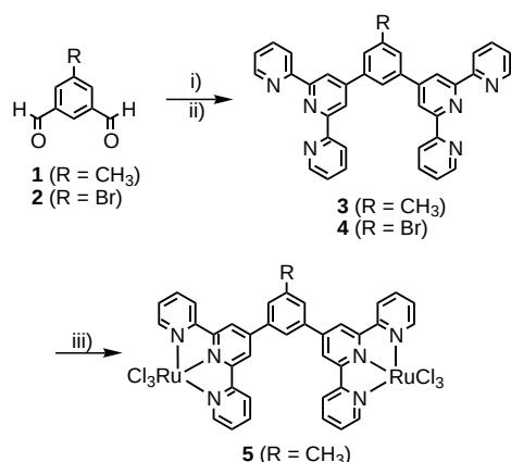
Scheme 1. Synthesis of the key monomers 3 , 4 , and bis( \text{Ru}^{\text{III}} ) adduct 5 : i) 2-acetylpyridine, NaOH, EtOH, 20 h, room temperature; ii) \text{AcO}^-\text{NH}_4^+ , AcOH, 4 h, reflux; iii) \text{RuCl}_3 \cdot 3\text{H}_2\text{O} , EtOH, 12 h, reflux.
