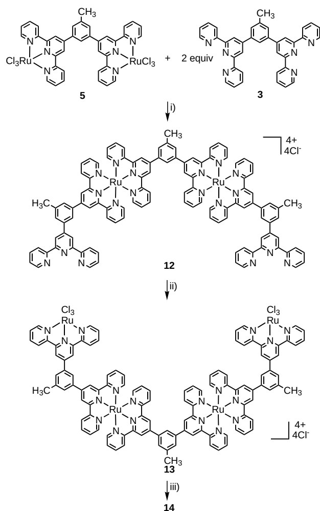
Scheme 5. Synthesis of trimeric precursors 12 and 13 for stepwise preparation of metallamacrocycle 14 : i) N -ethylmorpholine, MeOH, 12 h, reflux; ii) \text{RuCl}_3 \cdot 3\text{H}_2\text{O} , EtOH, 12 h, reflux; iii) a) 12 , N -ethylmorpholine, MeOH, 12 h, reflux, b) methanolic \text{NH}_4^+\text{PF}_6^- .
